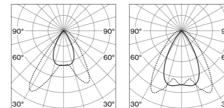
2 x 2 lamps 1 x shelf / 1 x wall floor washer
